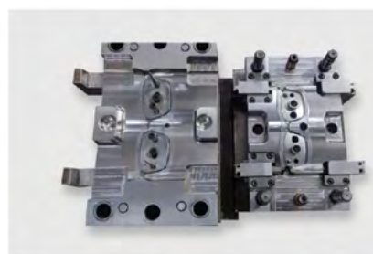
Frame moulding
