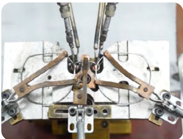
Frame welding
