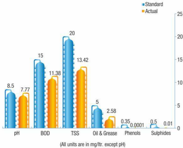
Treated Effluent Water Quality vis-a-vis Statutory Standards at Kochi Refinery
